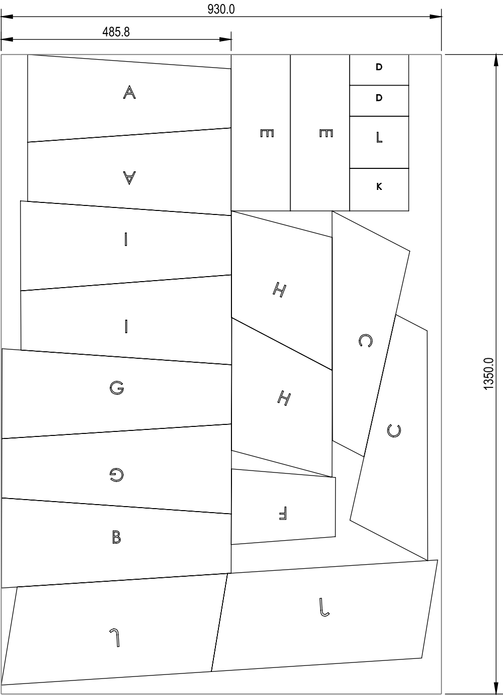
"DAMPING MATERIAL CUT PATTERN"
